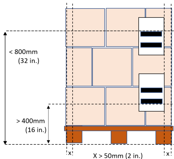
Figure 6.7.1.1-1. Barcode placement on pallets
