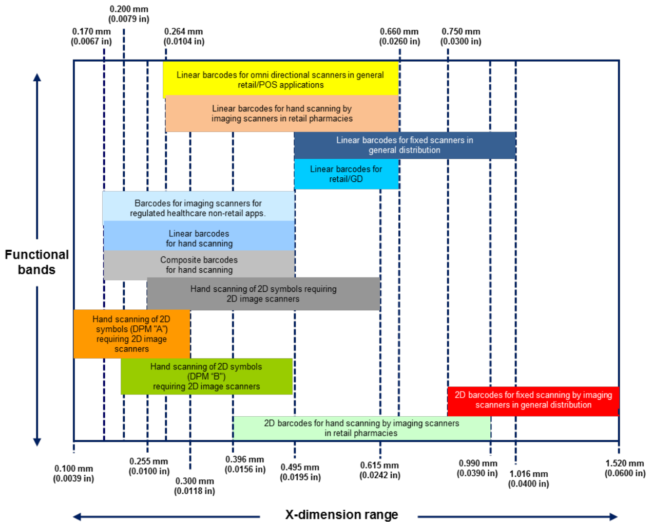
Figure 5.12.2.6-1. GS1 scanner functional operative bands
