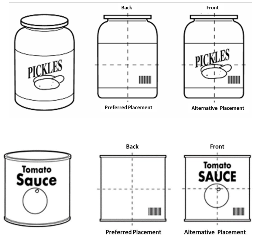
Figure 6.4.9-3. Barcode placement on large, heavy, or bulky jars, cans, jugs, or tubs
