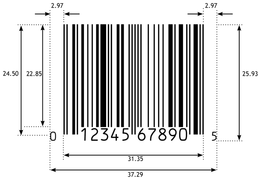
Figure 5.2.6.6-2. UPC-A barcode
