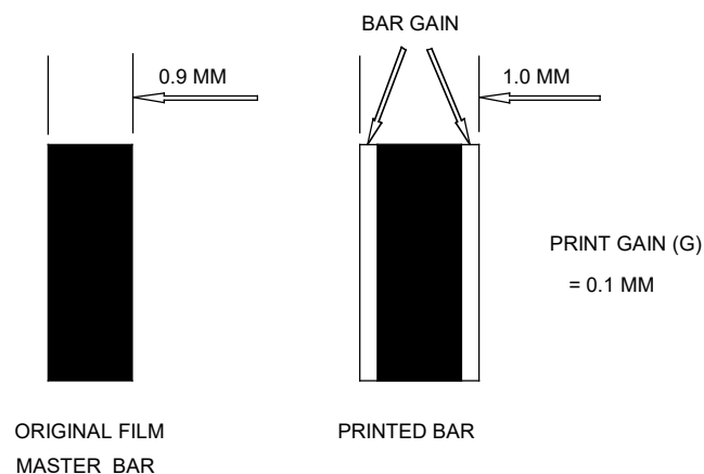
Figure 5.12.4.2.1-1. Example of bar width adjustment
