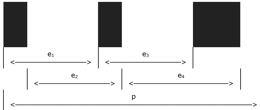
Figure 5.4.5-1. Decode measurements
