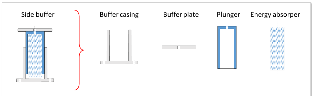
Figure 2.3.2-1. Example: Side buffer (assembly) with buffer casing (leading part)
