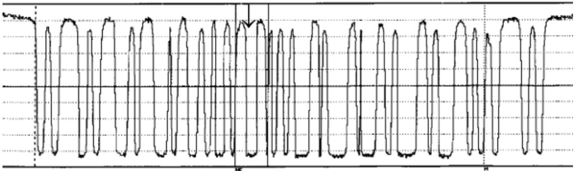
Figure 5.12.5.12-4. Scan Reflectance Profile of symbol with low decodability character
