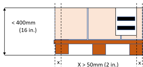
Figure 6.7.1.1-2. Barcode placement on pallets lower than 400 mm (16 inches)
