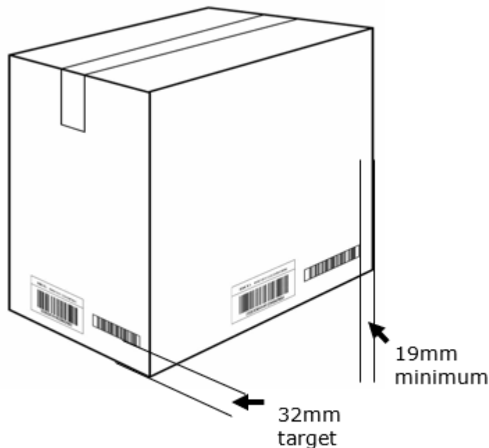
Figure 6.7.1.2-1. Barcode placement on cartons and outer cases
