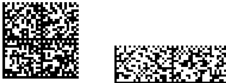
Figure 5.6.3.2-3. Segmented GS1 DataMatrix symbols: Square and rectangular formats (sizes of these GS1 DataMatrix symbols are larger than what would be used in a typical application so that typical alignment patterns can be easily seen.)
