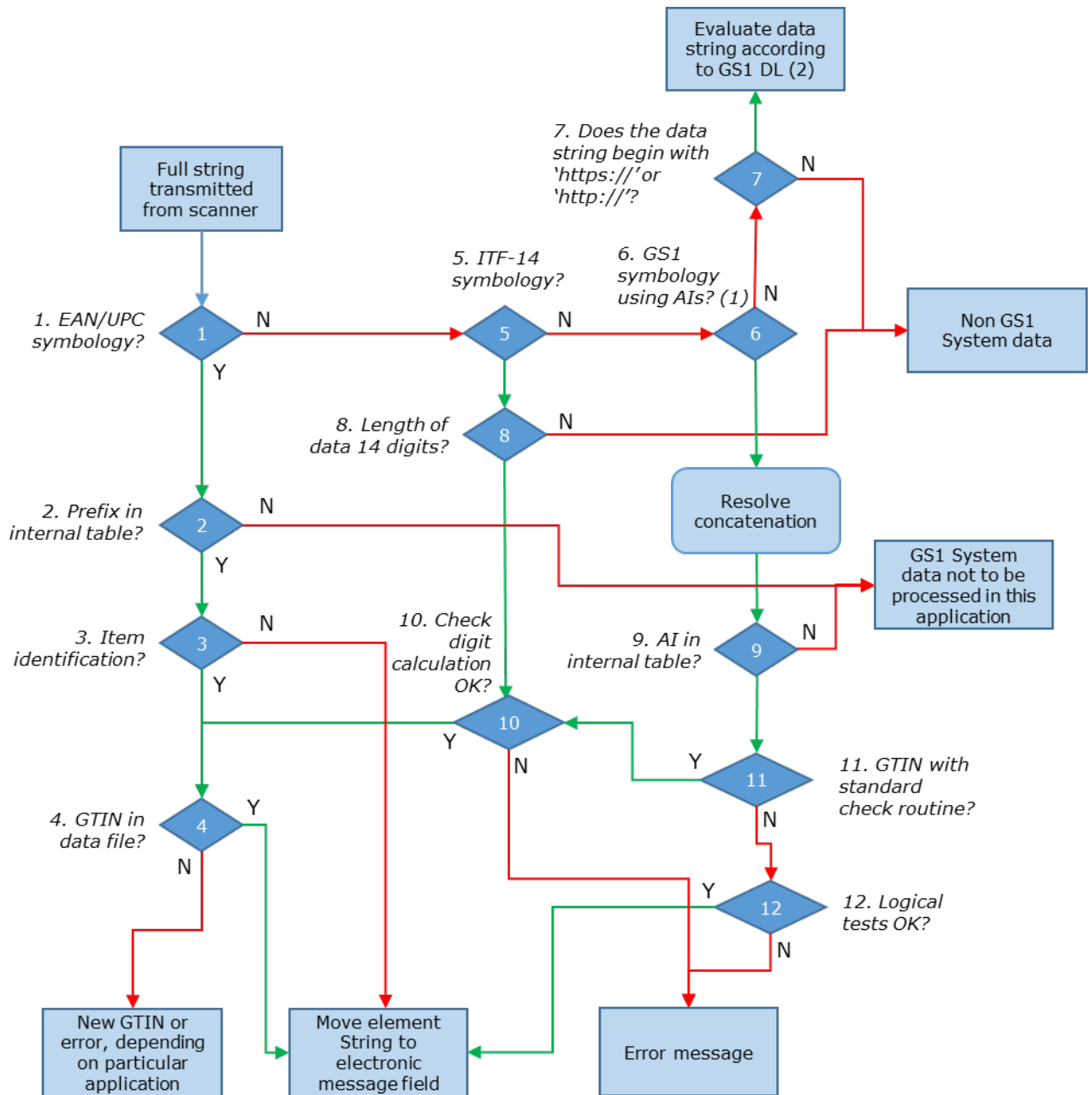
Figure 7.2.1-1. Test procedure
