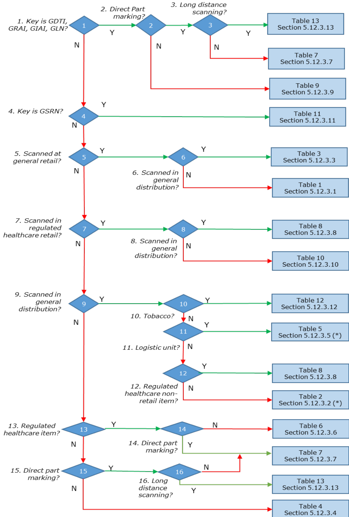
Figure 5.12.2.6-2. GS1 symbology operational environment decision tree
