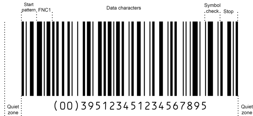
Figure 5.4.2-1. General format of a GS1-128 barcode
