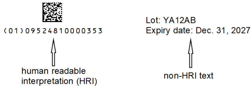
Figure 4.14-10. Example of human readable placement
