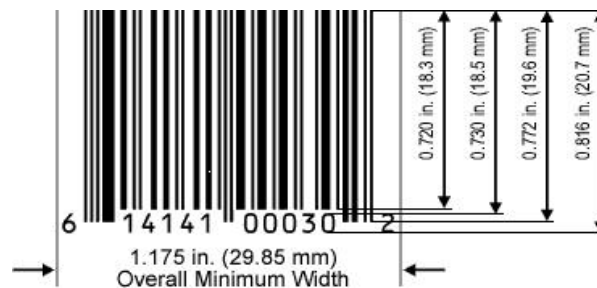
Figure 5.12.6.3-1. EAN/UPC symbol shown with minimum height and overall width dimensions for magnifications of 75 percent to 80 percent
