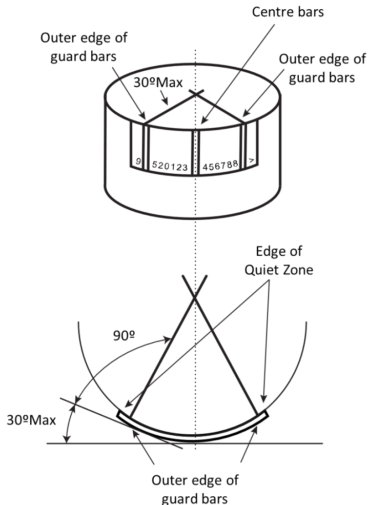
Figure 6.2.3.2-2. Relationship between symbol and curvature
