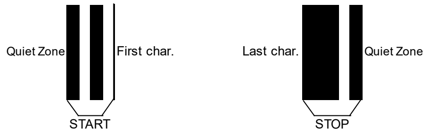
Figure 5.3.2.1.2-1. Start and stop patterns
